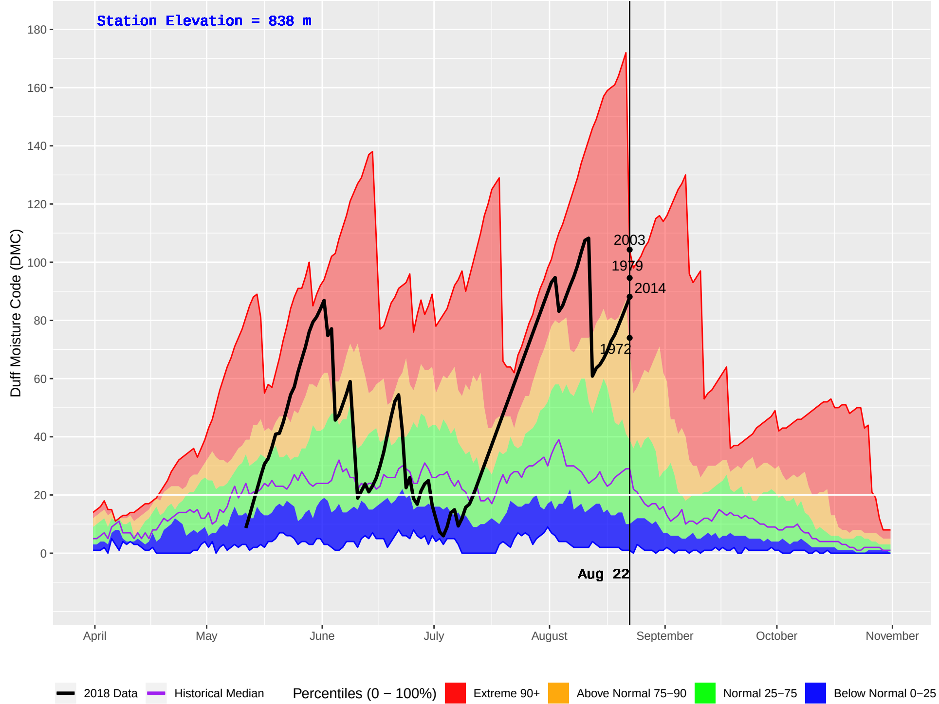
HOWARD (343) : Historical (1970–2016) and Current (2018) Daily Duff Moisture Code (DMC)
