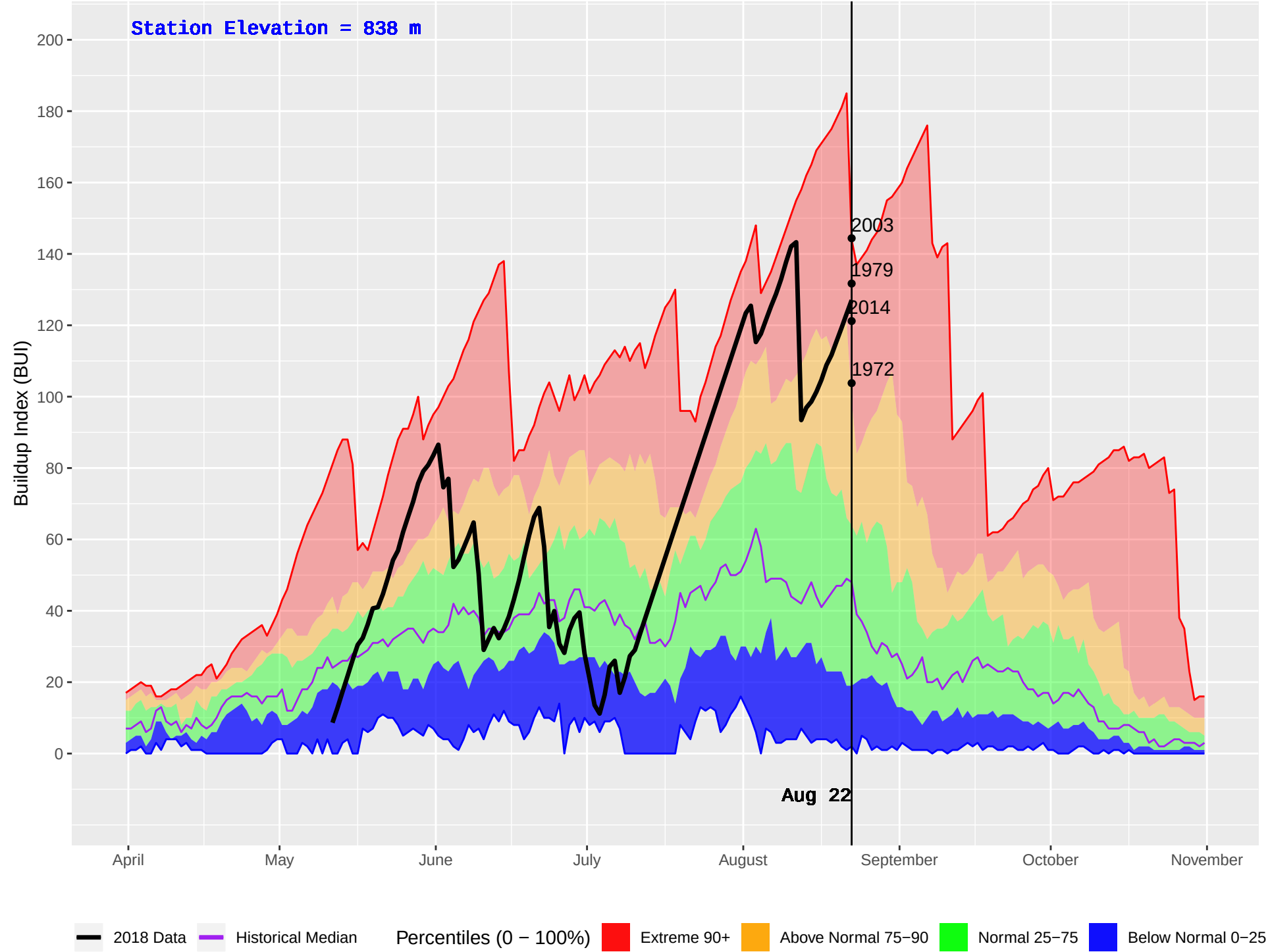
HOWARD (343) : Historical (1970–2016) and Current (2018) Daily Buildup Index (BUI)
