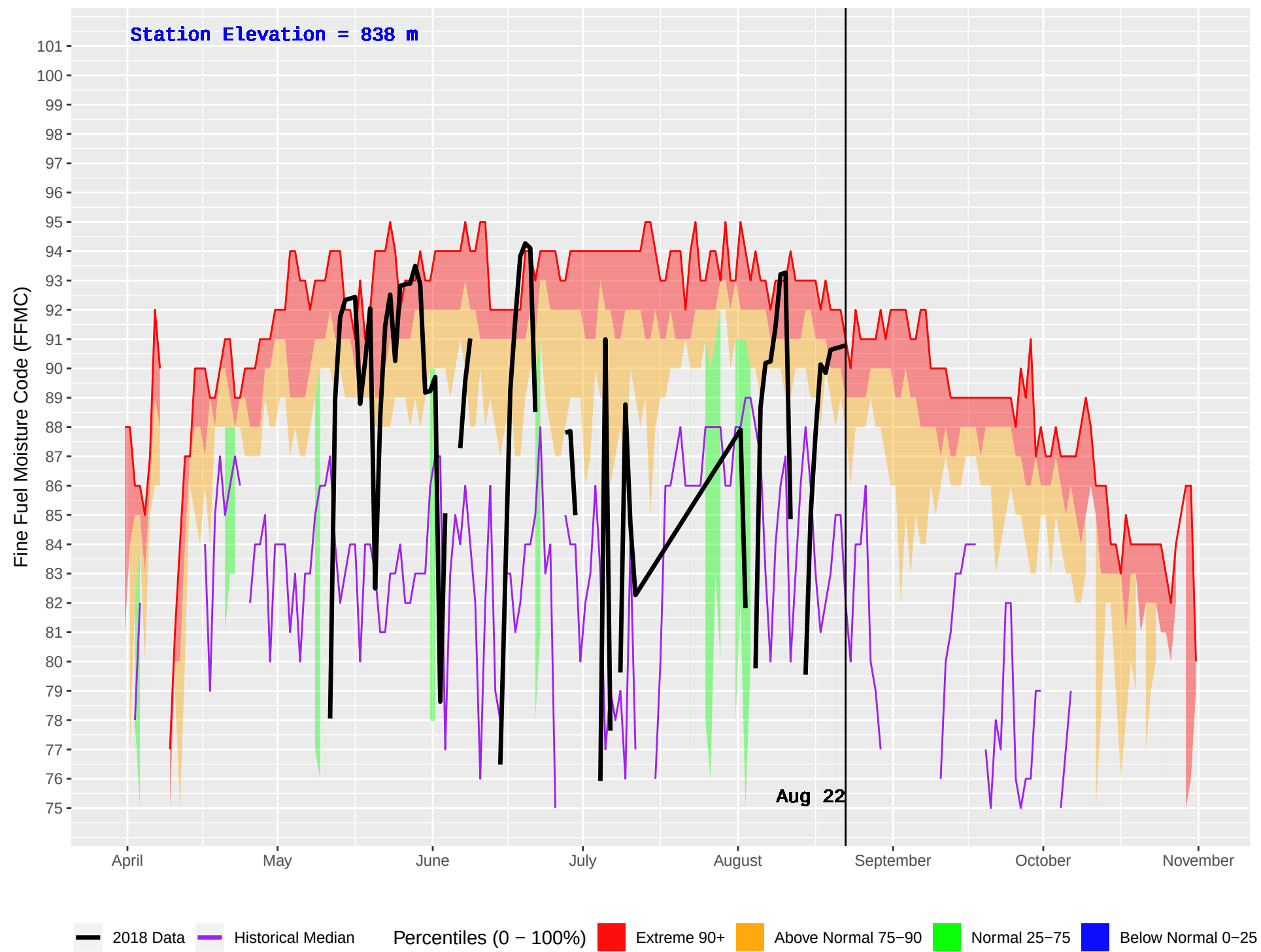
HOWARD (343) : Historical (1970–2016) and Current (2018) Daily Fine Fuel Moisture Code (FFMC)
