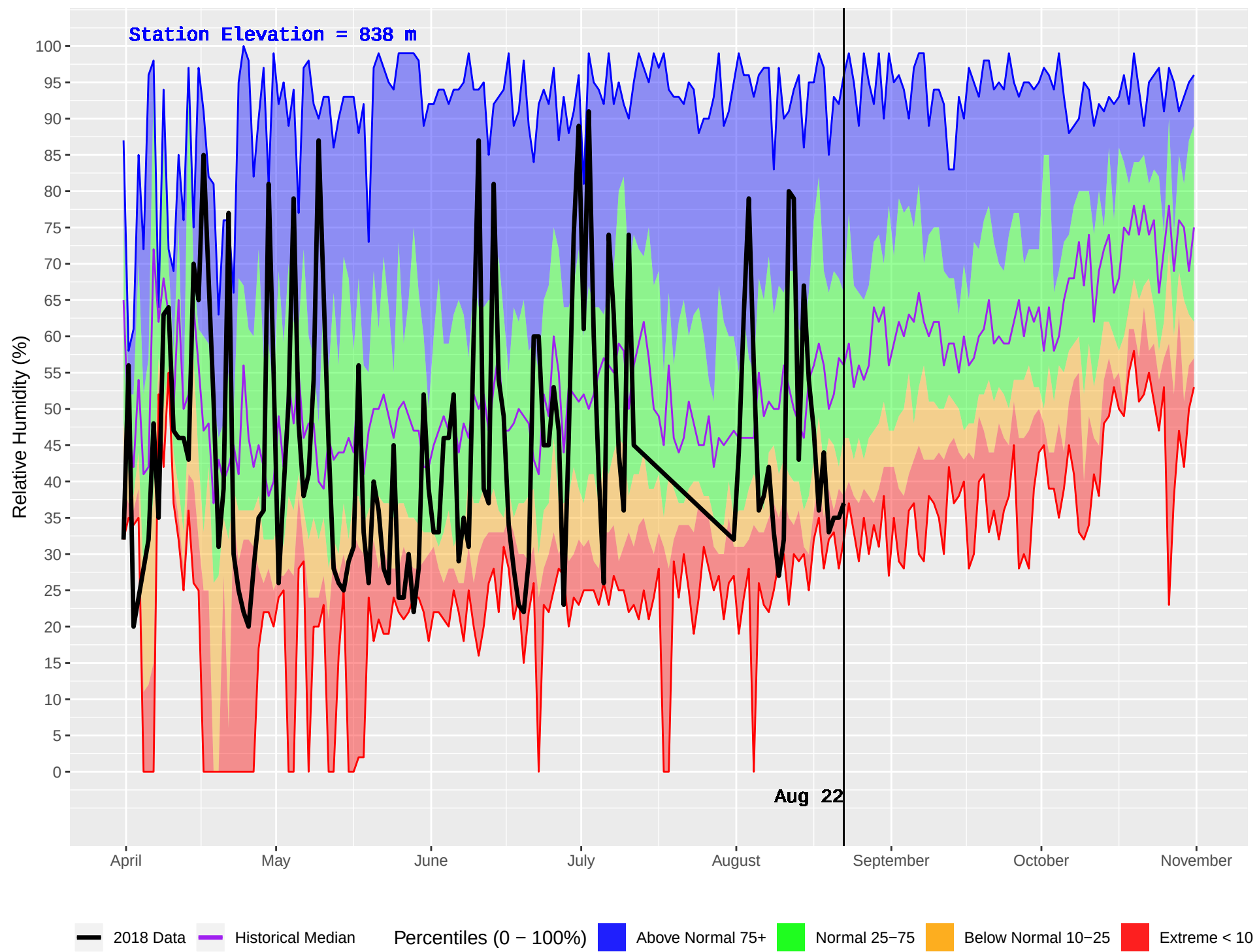
HOWARD (343) : Historical (1970–2016) and Current (2018) Daily Relative Humidity
