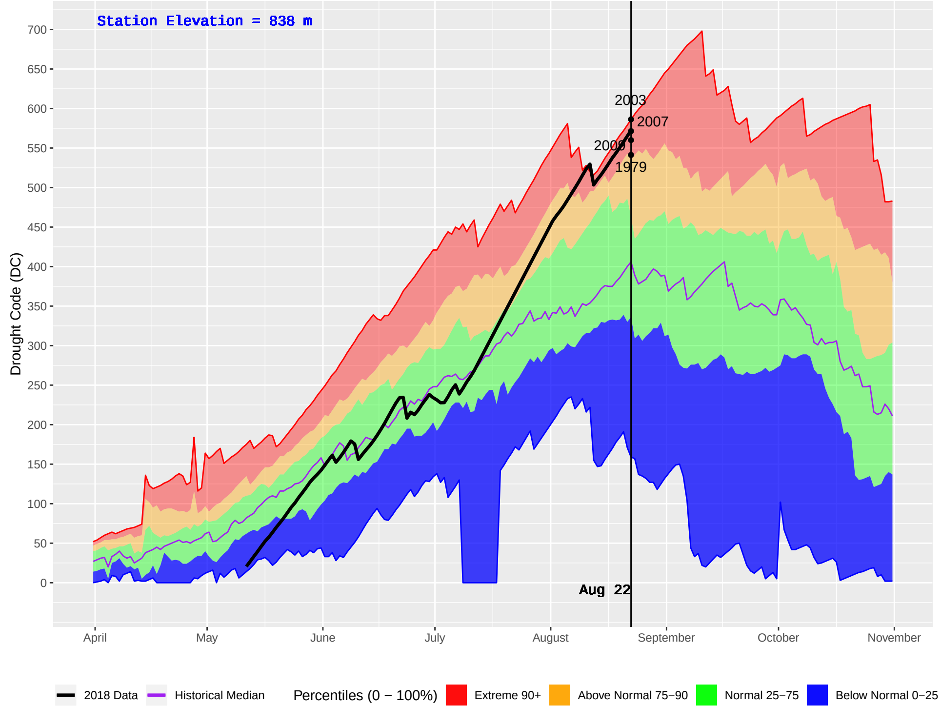
HOWARD (343) : Historical (1970–2016) and Current (2018) Daily Drought Code (DC)
