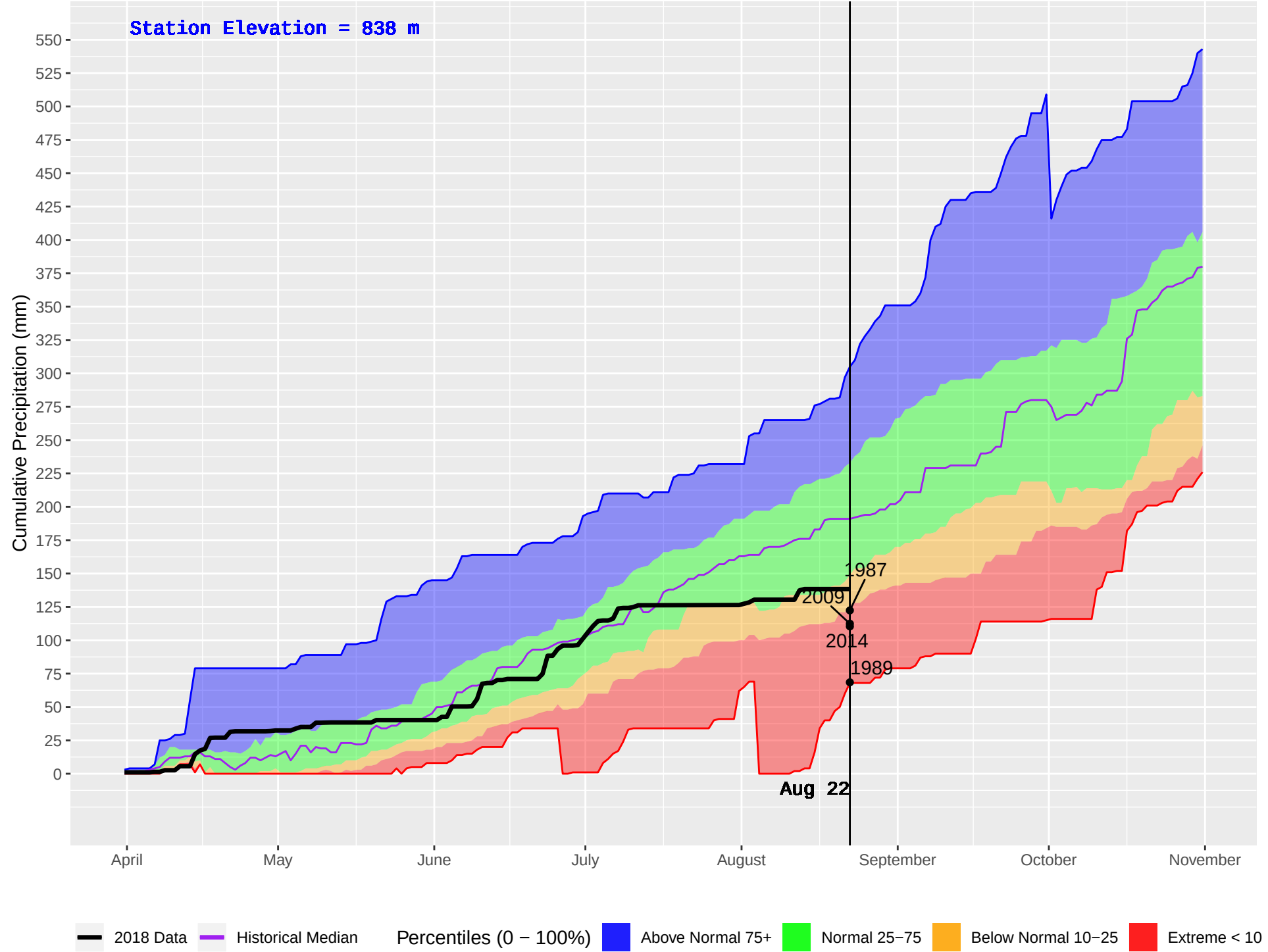
HOWARD (343) : Historical (1970–2016) and Current (2018) Daily Cumulative Precipitation
